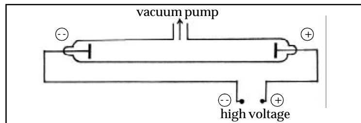
Discharge Tube
