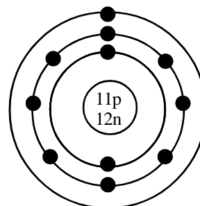
Model of Sodium atom
