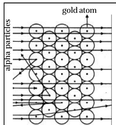
Deviation of alpha particles through gold foil
