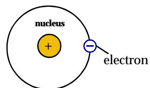
The atom model of Rutherford
